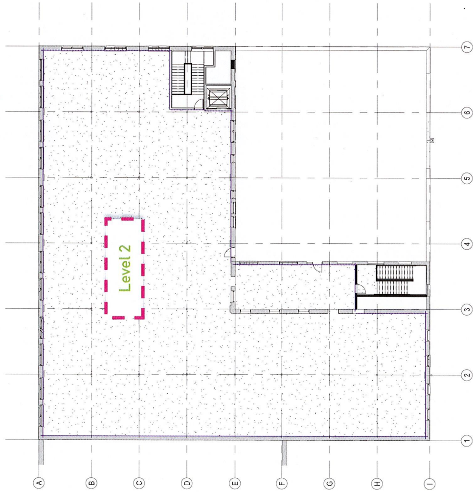
1 Level 2 - Area Plan AP-02 1" = 20'-0"
